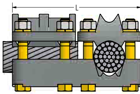
TAP CONFIGURATION
